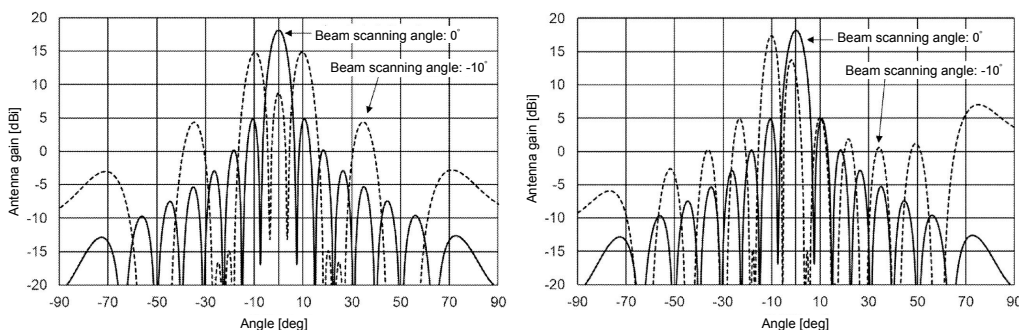
Fig. 1 Simulation results of directivity of the conventional (left) and novel (right) phased array antenna systems
